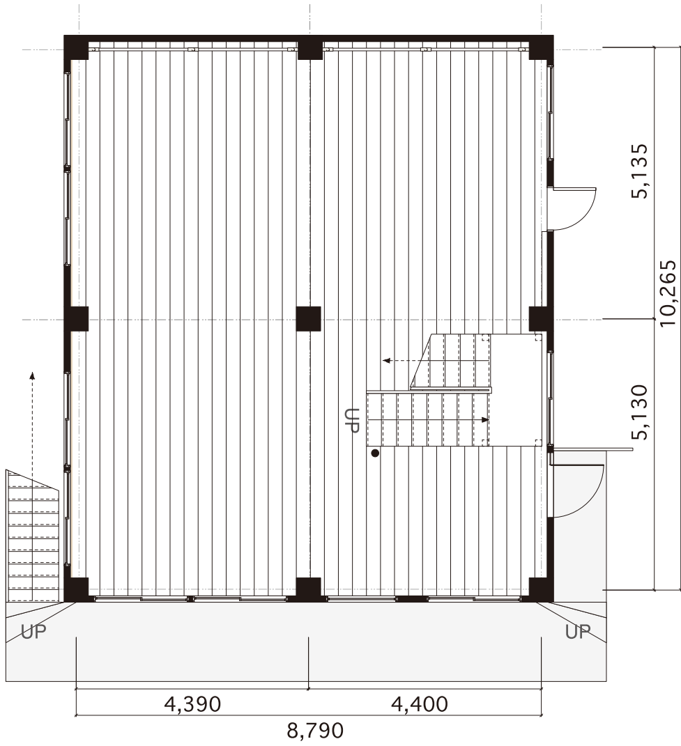
1F(90m 2 )
