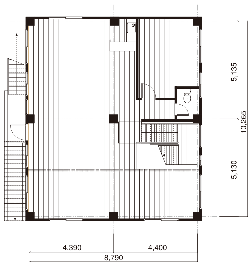
2F(90m 2 )
