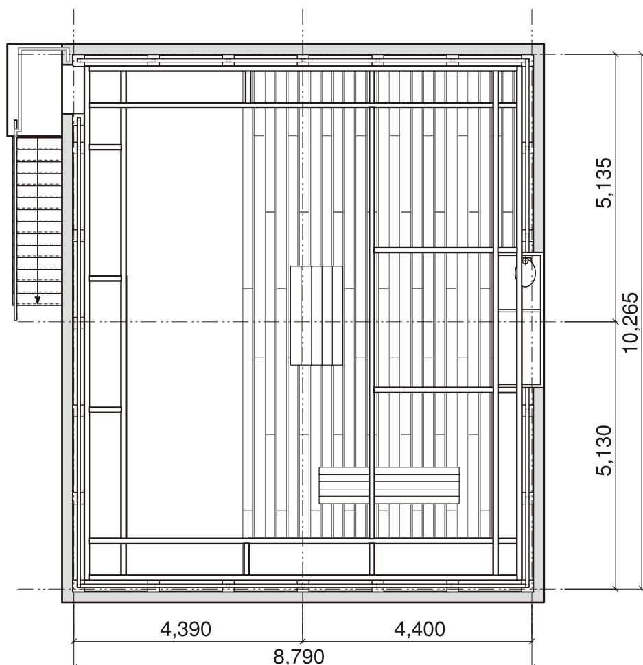
ROOF(90m 2 )
